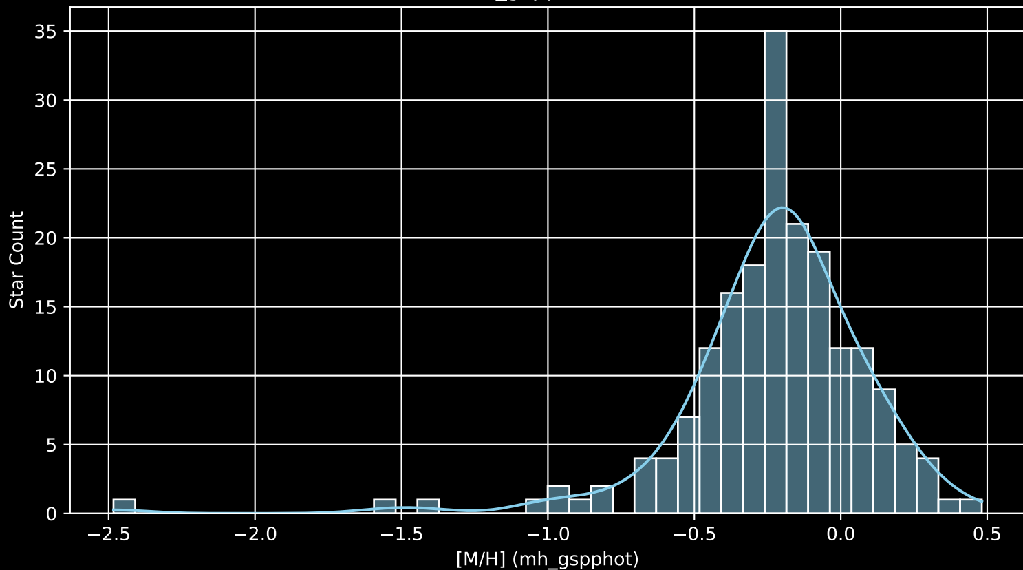
APOGEE DR17 Field: [CVZ_OB18_btx [M/H] (mh_gspphot) (n= 189)
