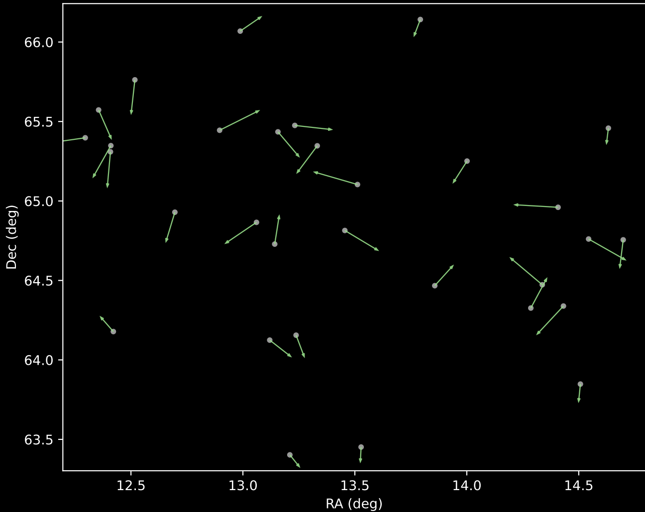
APOGEE DR17 Cluster 5 Proper Motion Vectors (n=31)
