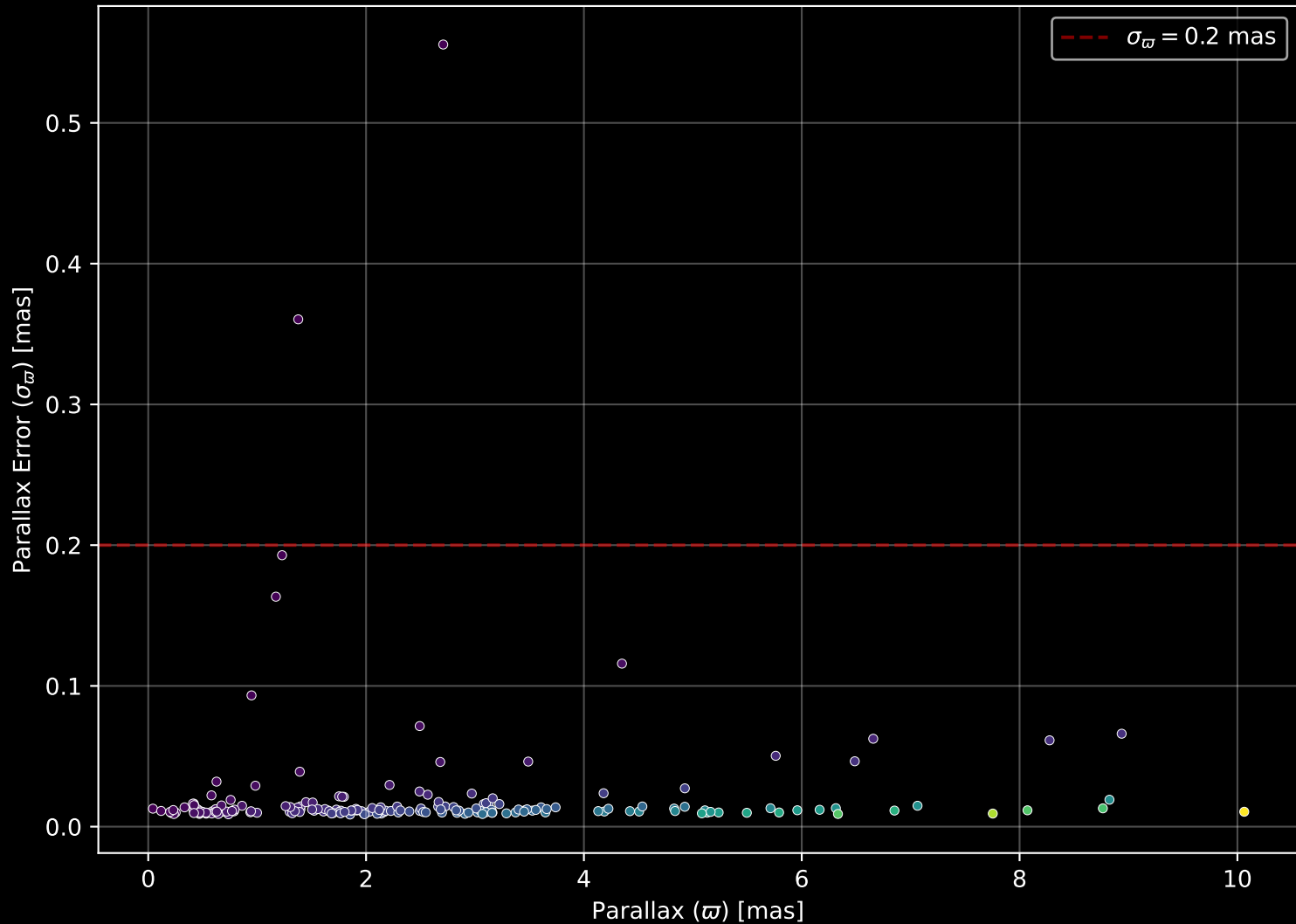
APOGEE DR17 Field: [CVZ_OB18_btx] Parallax Quality (n= 190)
