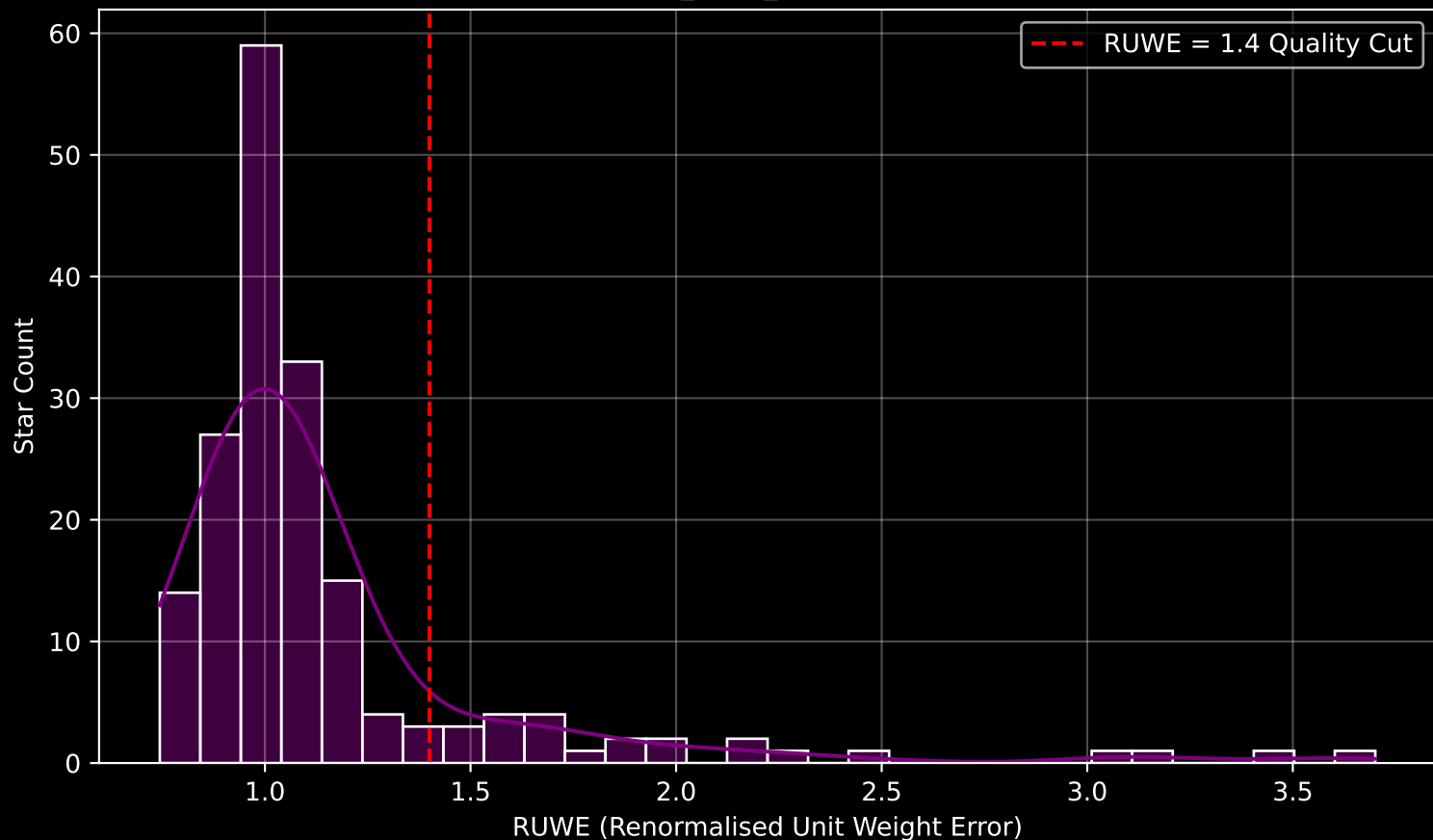
GAPOGEE DR17 Field [CVZ_OB18_btx] RUWE Distribution (n= 179)
