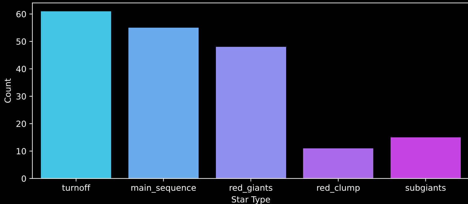
APOGEE DR17 Field: [CVZ_OB18_btx] Count plot of Star Type
