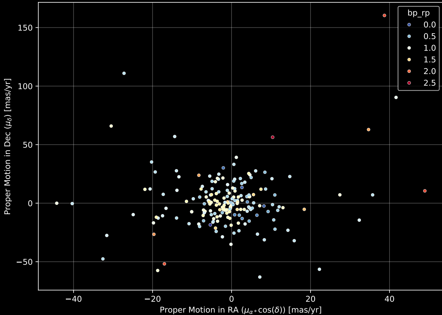
APOGEE DR17 Field: [CVZ_OB18_btx] Proper Motion Diagram (n= 190)
